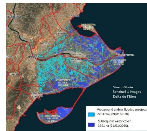
Earth Observation
